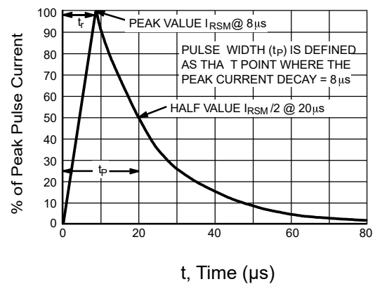
Figure 4: 8 X 20 \mu s Pulse Waveform
