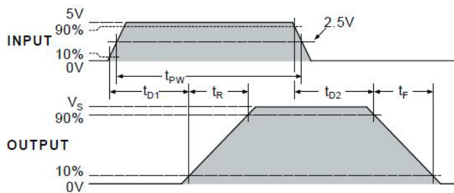
Figure 2. Input-Output B Functionality Diagram
