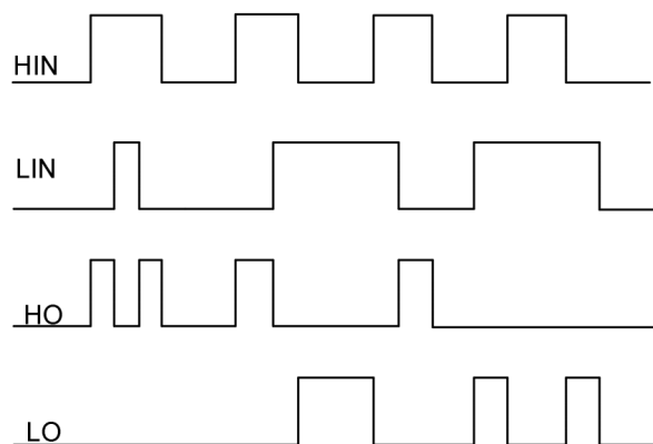
Figure 1. UMW IRS2304STR Input and output timing waveform
