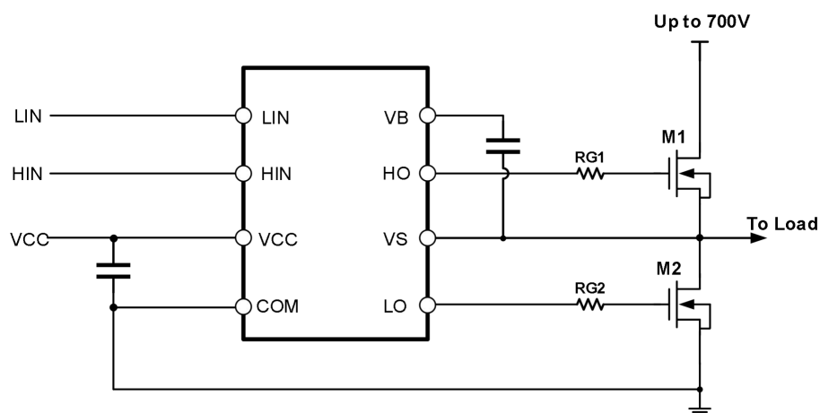
Figure 5. Typical application circuit of UMW IRS2304STR
