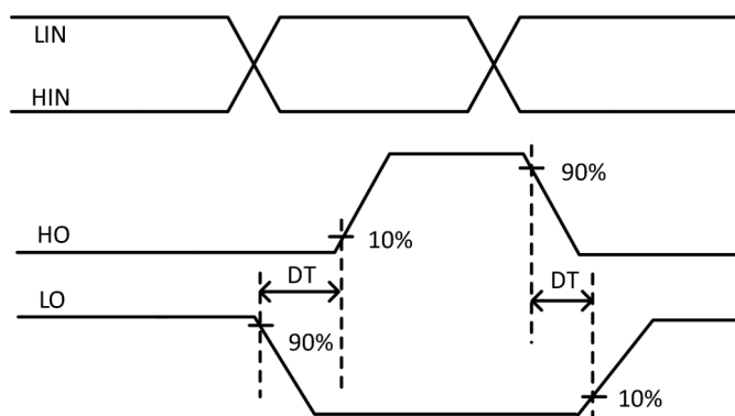
Figure 3. Cross Conduction Prevention Delay Time Waveform Definition
