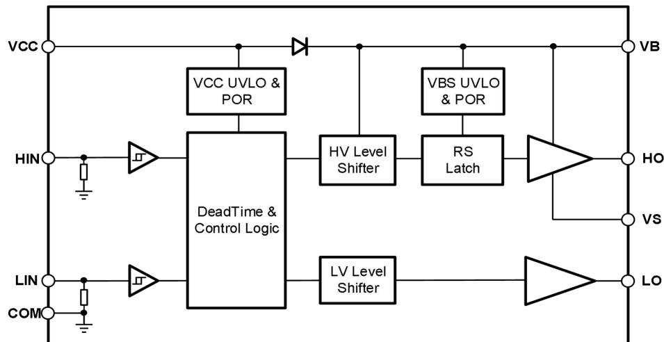
Figure 4. Function Block Diagram of UMW IRS2304STR
