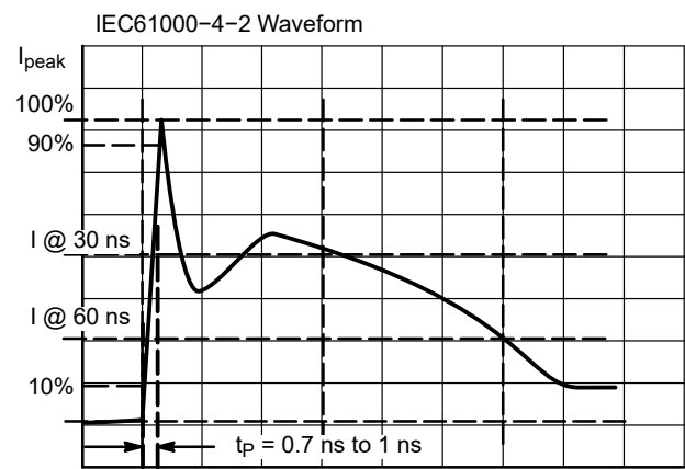
Figure 7: IEC61000-4-2 Spec
