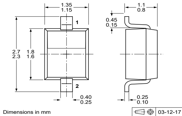
PESD5V0L1UA (SOD323)
