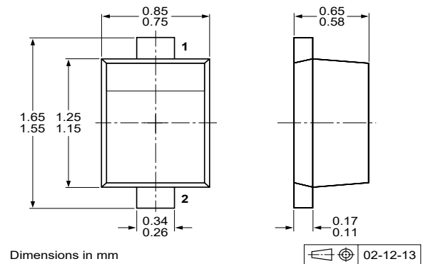
PESD5V0L1UB (SOD523)
