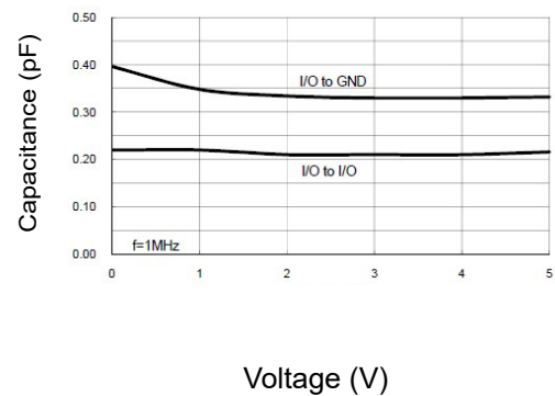
Figure 4: C-Voltage vs Capacitance
