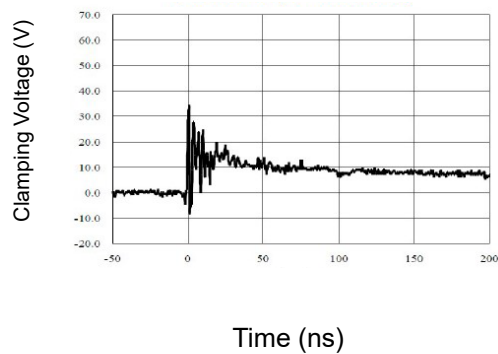
Figure 5: ESD Clamping of I/O to GND (+8kV Contact per IEC 61000-4-2)
