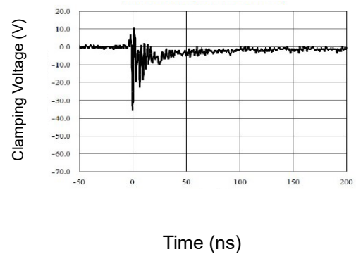
Figure 6: ESD Clamping of I/O to GND (-8kV Contact per IEC 61000-4-2)
