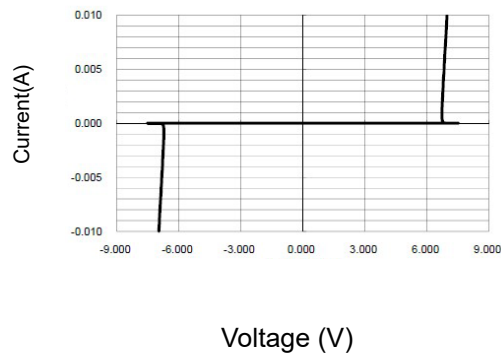
Figure 3: Voltage Sweeping of I/O to I/O
