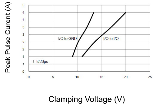
Figure 2: Clamping Voltage vs Peak Pulse Current
