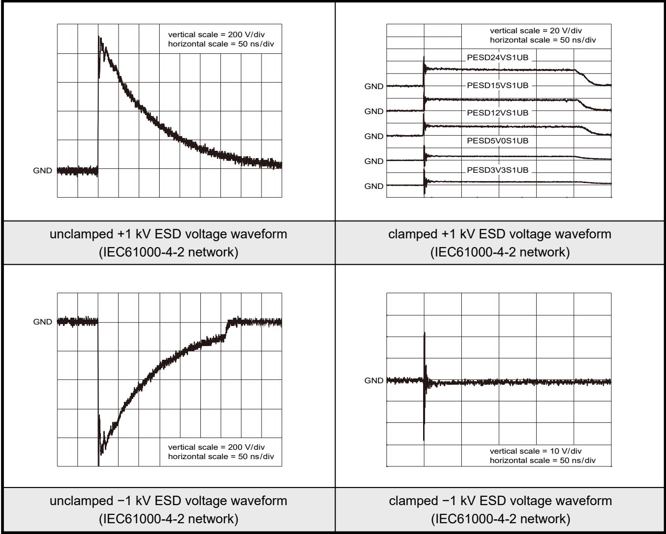
Figure 8: ESD clamping test setup and waveforms
