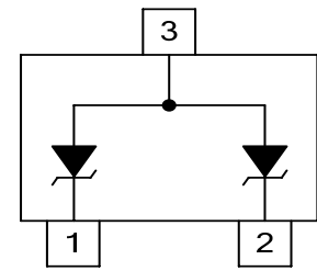
Pin Configuration
