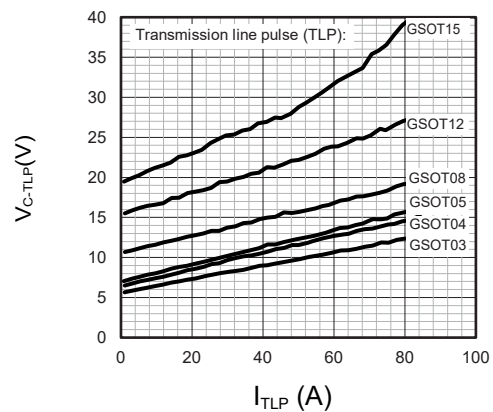
Figure 6: Typical Clamping Voltage vs. Peak Pulse Current
